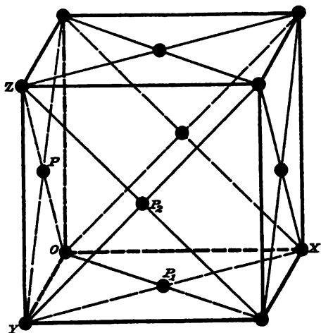
FIG. 31. A rectangular parallelepiped. If YZ \neq YO \neq OX it corresponds to \Gamma_0'' , if YZ \neq YO = OX to \Gamma_1'(a) , or if YZ = YO = OX to \Gamma_1' .
